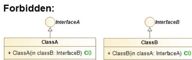
Figure 2.6.: Forbidden circular dependency
