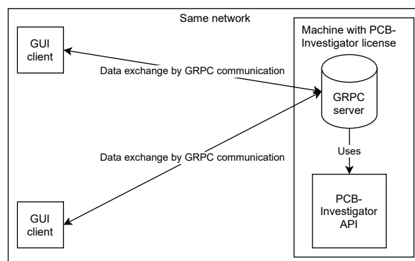
Figure 3.1.: Client-server structure of the planned software
