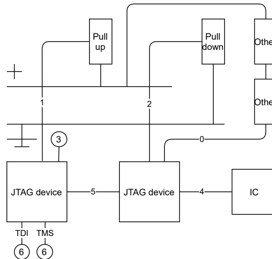
Figure 4.7.: The determined pin types of interest
