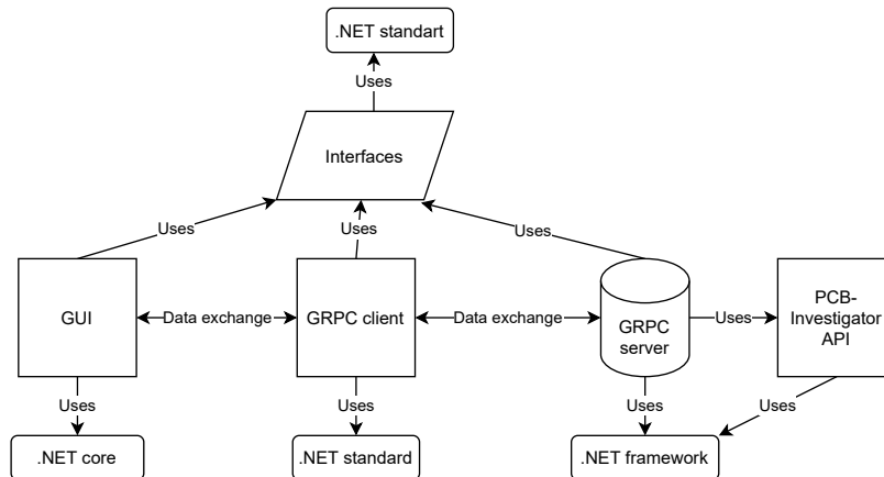
Figure 3.2.: Frameworks used within the project
