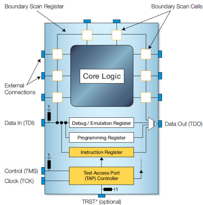
Figure 2.3.: JTAG interface in detail[5]
