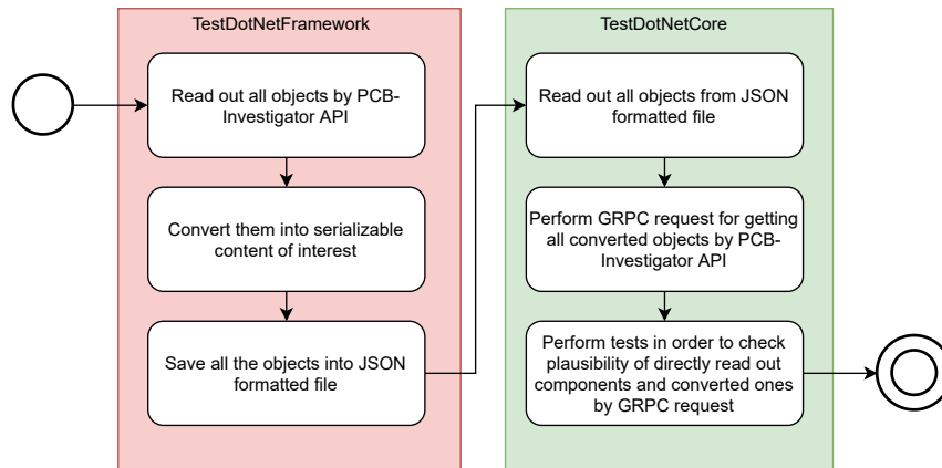
Figure 4.9.: The sequence for a complete test of parsing validation of objects received by PCB-Investigator API
