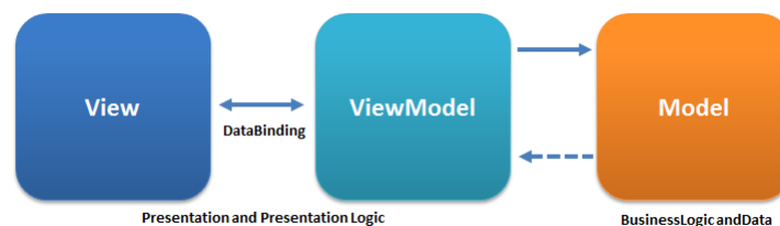
Figure 2.5.: MVVM structure [14]
